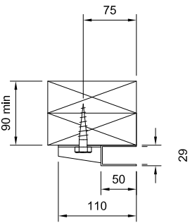
TYPICAL TIMBER FIXING (BY OTHERS)
