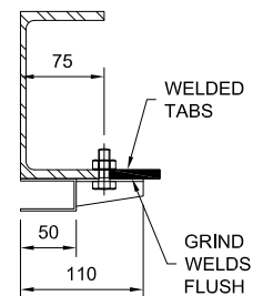
TYPICAL STEEL FIXING (BY OTHERS)
