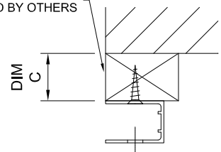
TIMBER PACKERS SUPPLIED AND FITTED BY OTHERS FACE FIX GUIDE
