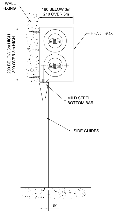
SECTION THROUGH HEAD BOX
